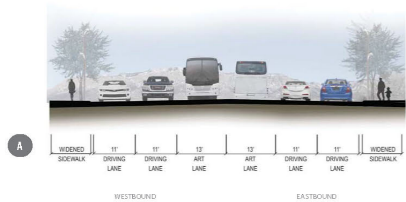
CROSS SECTION BETWEEN SIMONDS ST AND CLAYTON ST
