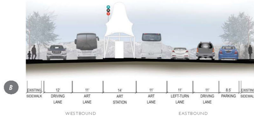
CROSS SECTION AT WASHINGTON STATION
