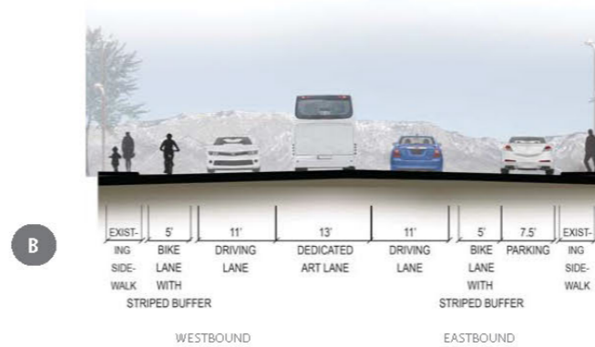
CROSS SECTION BETWEEN RANCHO SECO RD AND LAGUNA BLVD
