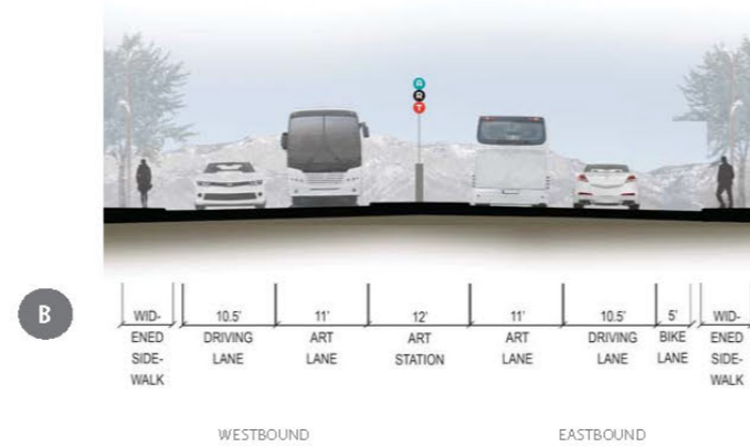
CROSS SECTION AT WALTER STATION
