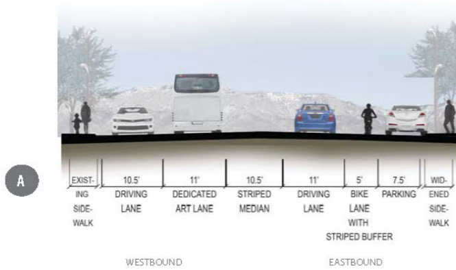
CROSS SECTION BETWEEN ARNO ST AND EDITH BLVD
