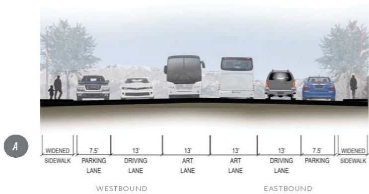
CROSS SECTION BETWEEN TULANE DR AND AMHERST DR
